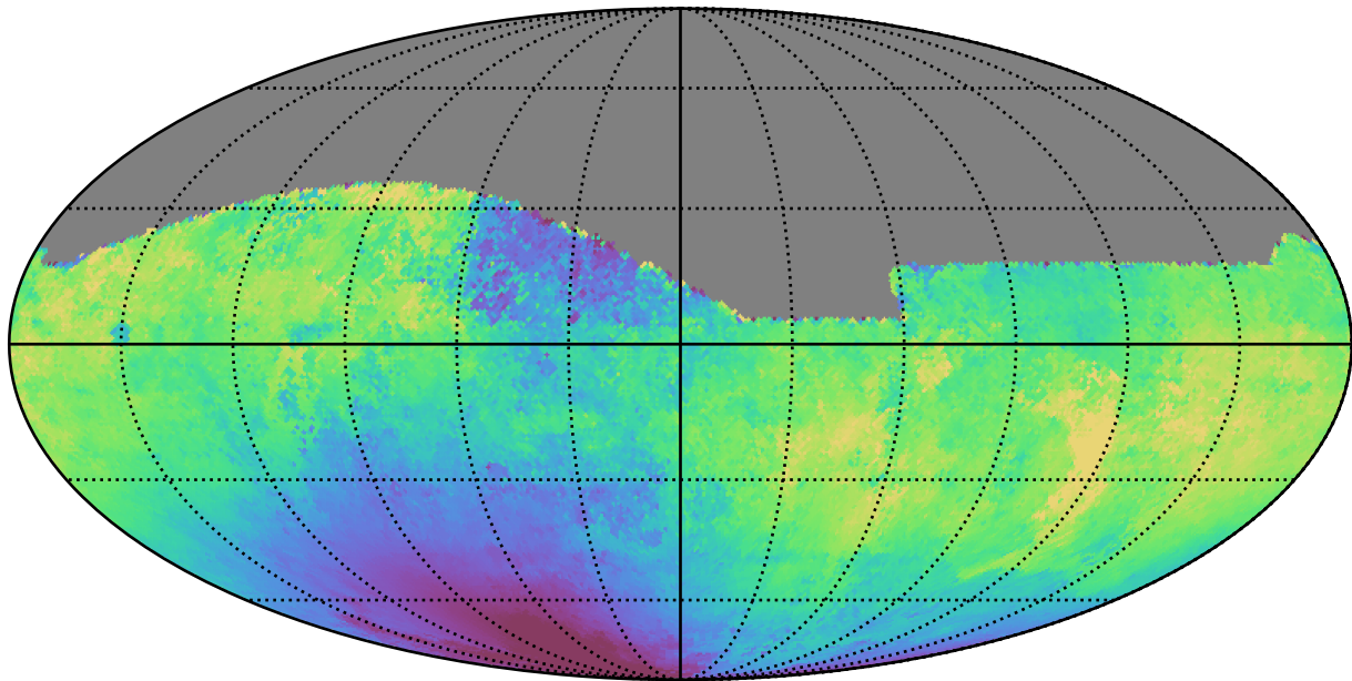
weather_cloudso8v3.4_10yrs All sky g band: Median solarElong
