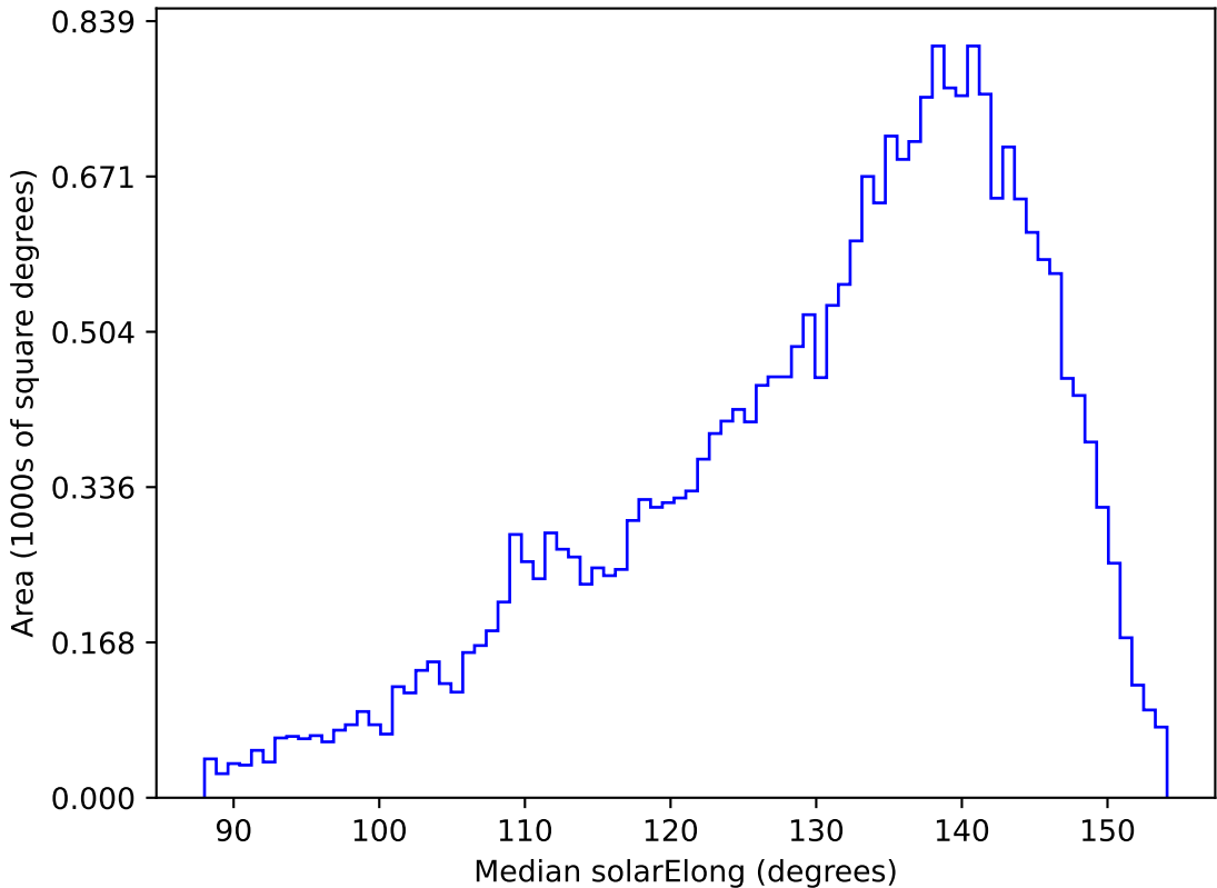
weather_cloudso8v3.4_10yrs All sky g band: Median solarElong
