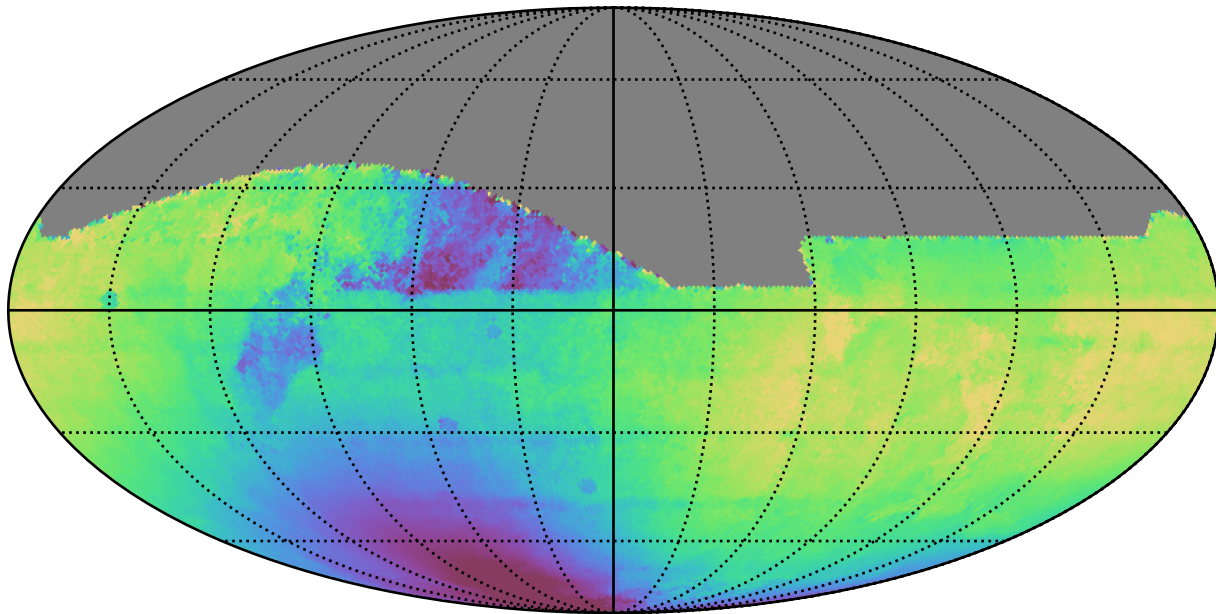
weather_cloudso8v3.4_10yrs All sky all bands: Median solarElong
