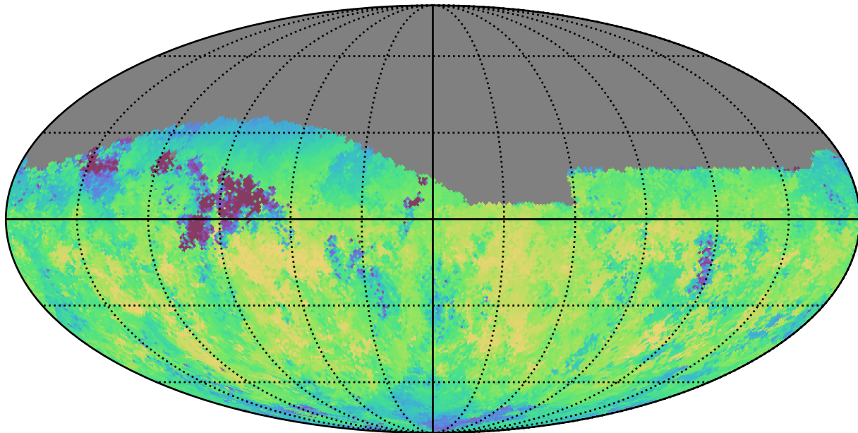
weather_cloudso8v3.4_10yrs Yr 1 z band: Median skyBrightness
