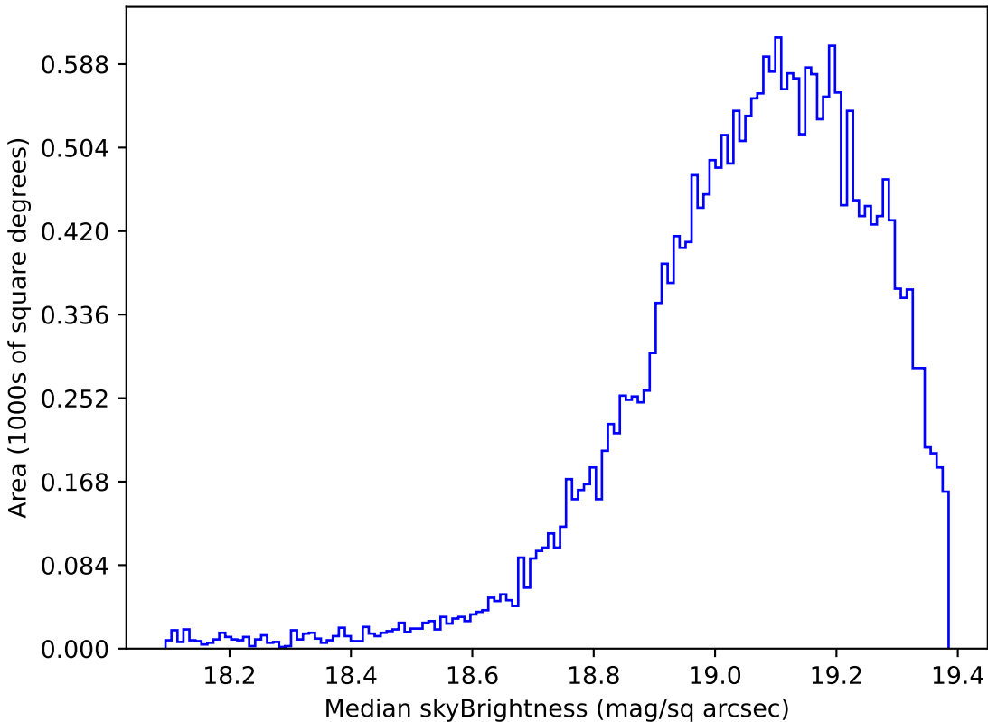
weather_cloudso8v3.4_10yrs Yr 1 z band: Median skyBrightness
