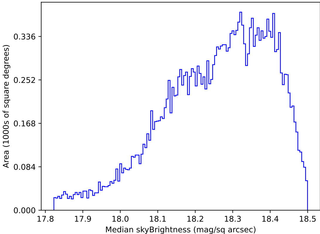
weather_cloudso8v3.4_10yrs Yr 1 y band: Median skyBrightness
