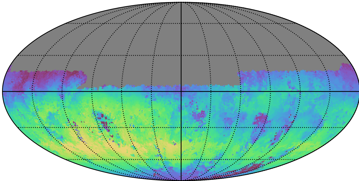
weather_cloudso8v3.4_10yrs Yr 1 u band: Median skyBrightness
