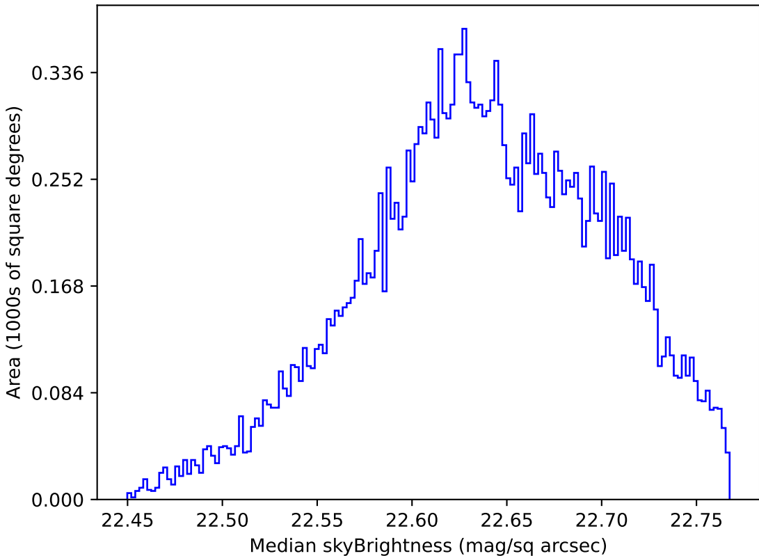
weather_cloudso8v3.4_10yrs Yr 1 u band: Median skyBrightness
