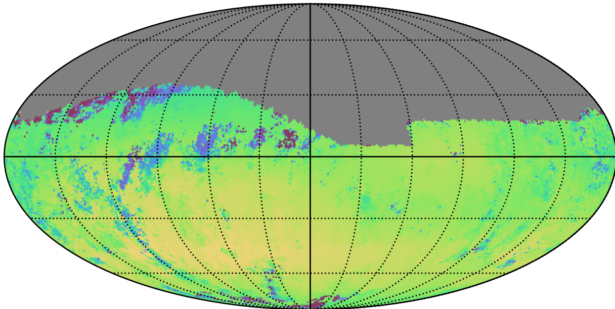
weather_cloudso8v3.4_10yrs Yr 1 r band: Median skyBrightness
