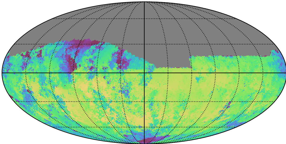
weather_cloudso8v3.4_10yrs Yr 1 i band: Median skyBrightness
