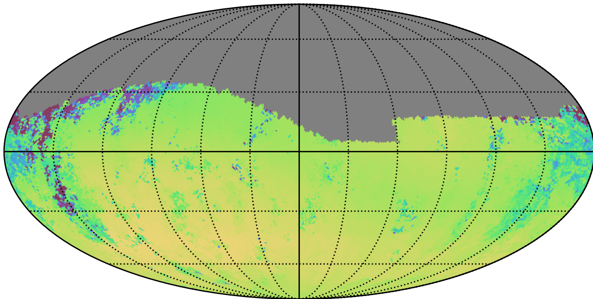
weather_cloudso8v3.4_10yrs Yr 1 g band: Median skyBrightness
