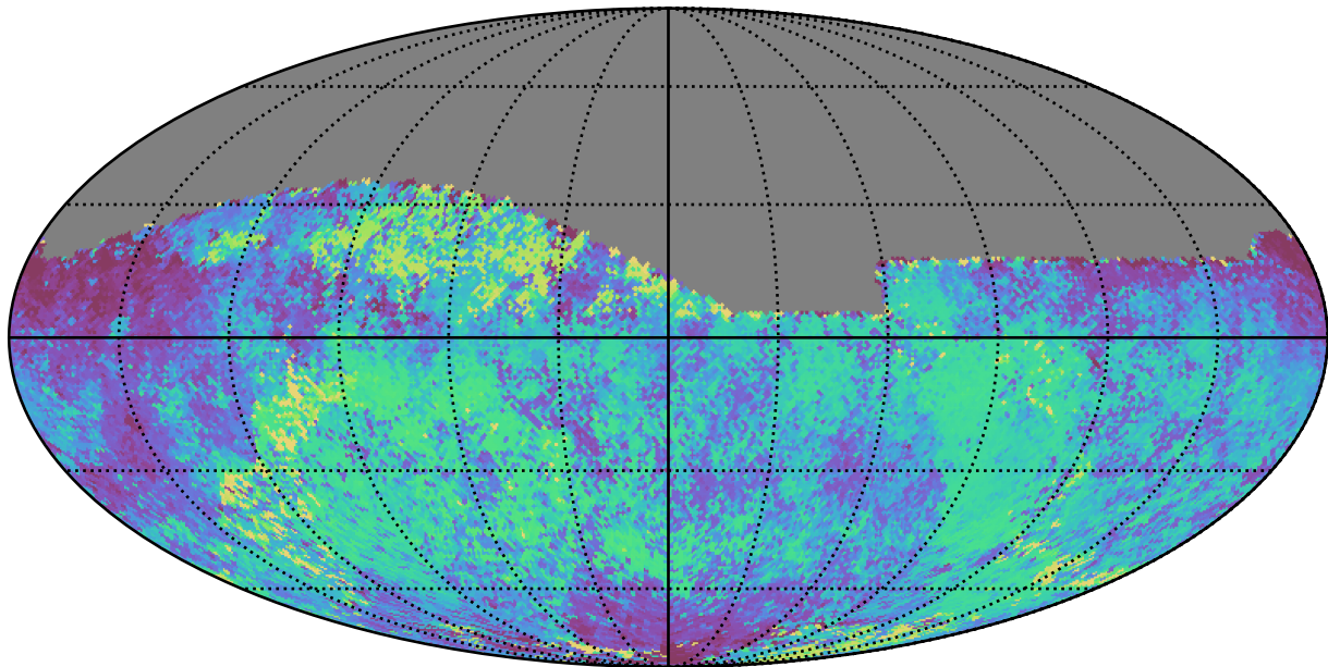
weather_cloudso8v3.4_10yrs Yr 1 all bands: Median skyBrightness
