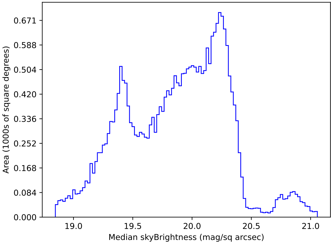
weather_cloudso8v3.4_10yrs Yr 1 all bands: Median skyBrightness
