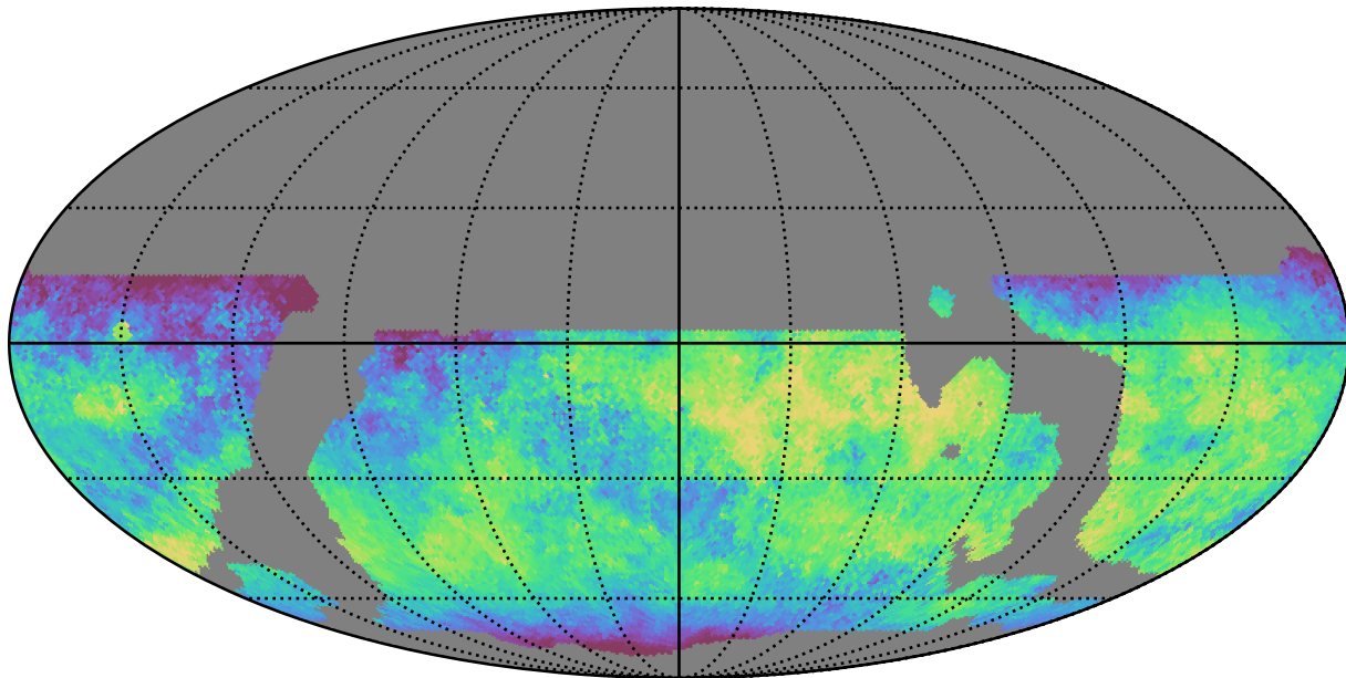
weather_cloudso8v3.4_10yrs WFD z band: Median skyBrightness
