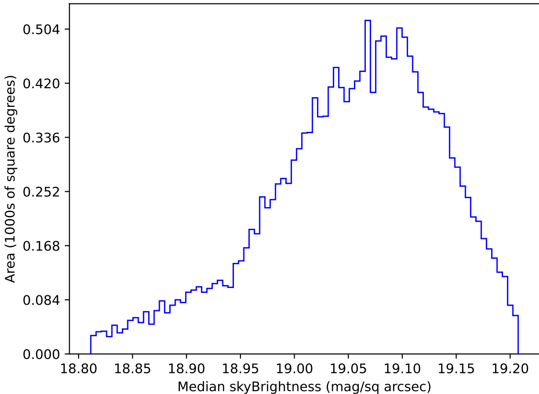
weather_cloudso8v3.4_10yrs WFD z band: Median skyBrightness
