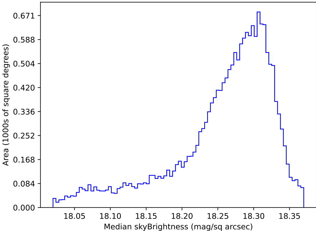
weather_cloudso8v3.4_10yrs WFD y band: Median skyBrightness
