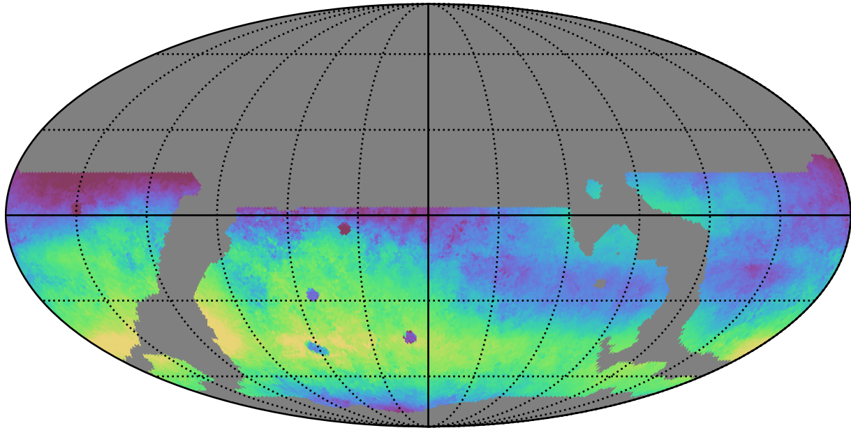
weather_cloudso8v3.4_10yrs WFD r band: Median skyBrightness
