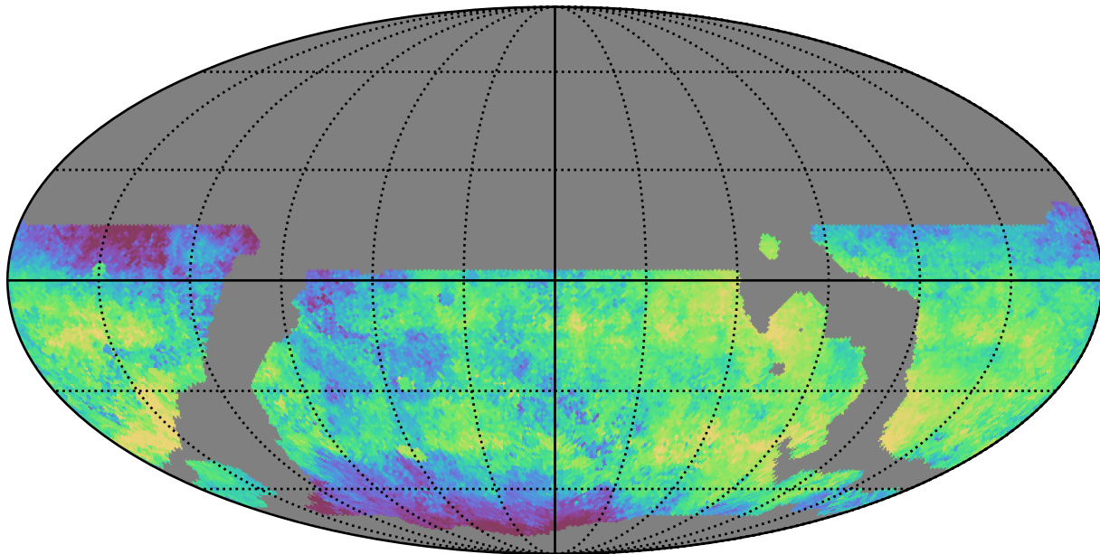
weather_cloudso8v3.4_10yrs WFD i band: Median skyBrightness
