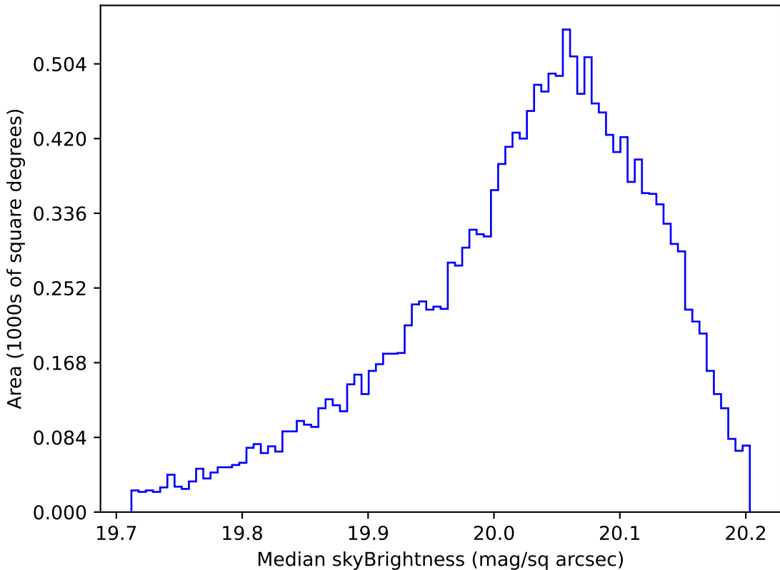
weather_cloudso8v3.4_10yrs WFD i band: Median skyBrightness
