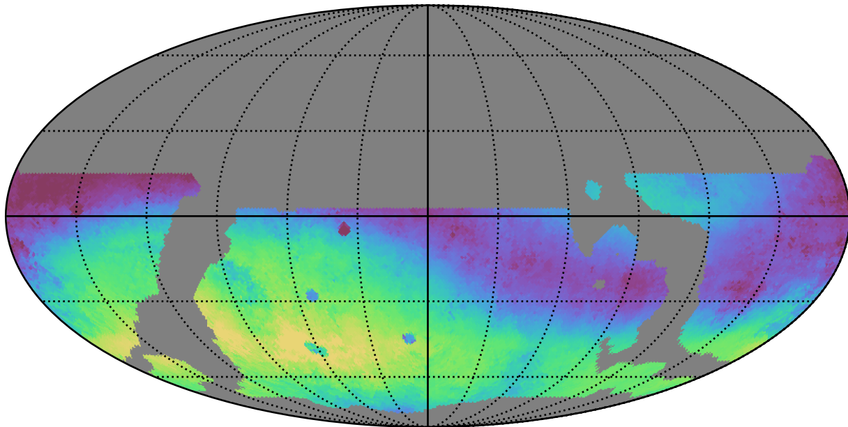
weather_cloudso8v3.4_10yrs WFD g band: Median skyBrightness
