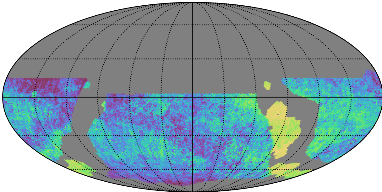
weather_cloudso8v3.4_10yrs WFD all bands: Median skyBrightness
