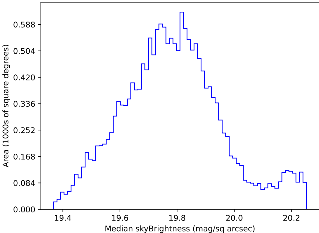
weather_cloudso8v3.4_10yrs WFD all bands: Median skyBrightness
