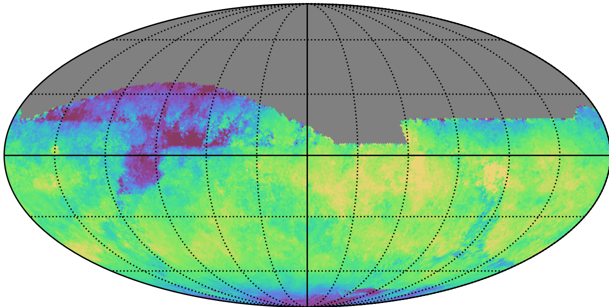
weather_cloudso8v3.4_10yrs All sky z band: Median skyBrightness
