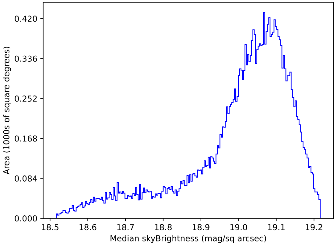
weather_cloudso8v3.4_10yrs All sky z band: Median skyBrightness
