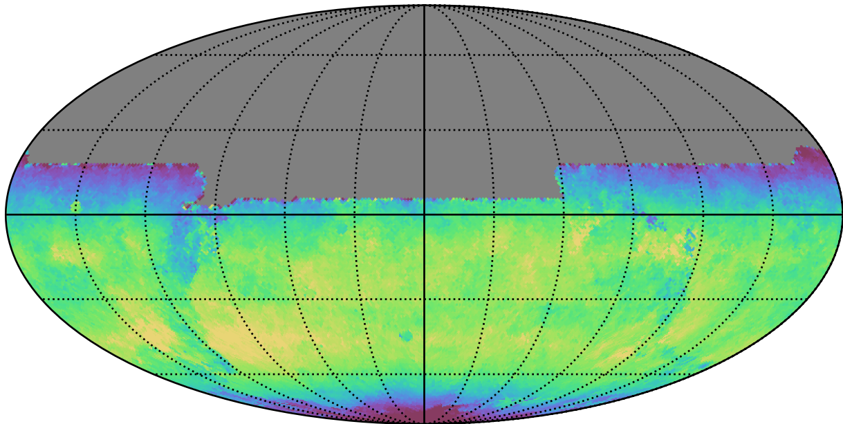
weather_cloudso8v3.4_10yrs All sky y band: Median skyBrightness
