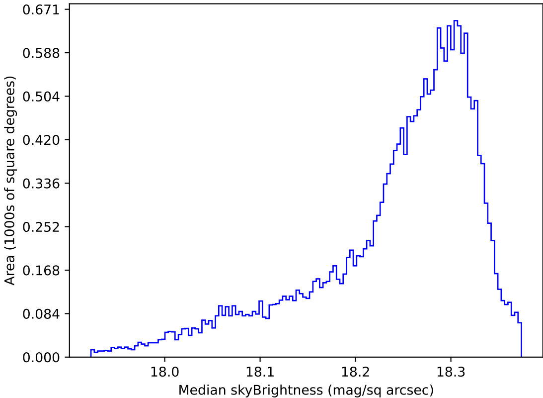
weather_cloudso8v3.4_10yrs All sky y band: Median skyBrightness
