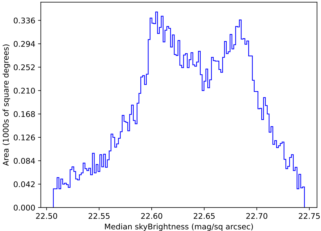
weather_cloudso8v3.4_10yrs All sky u band: Median skyBrightness
