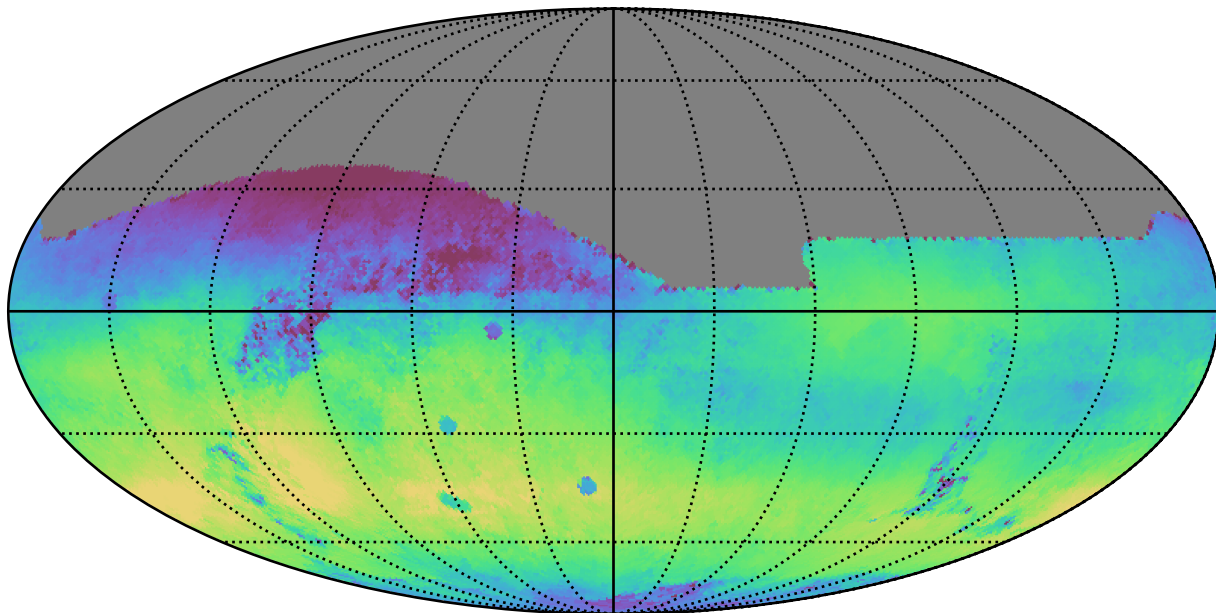
weather_cloudso8v3.4_10yrs All sky r band: Median skyBrightness
