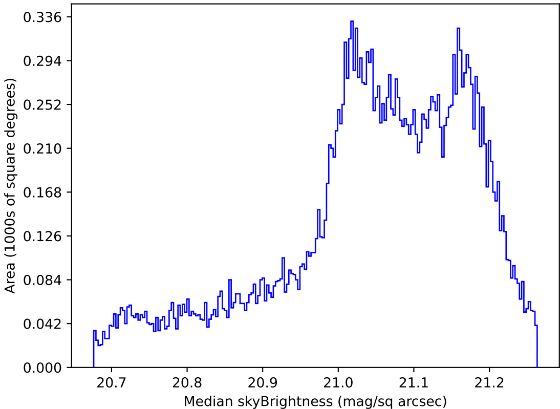
weather_cloudso8v3.4_10yrs All sky r band: Median skyBrightness
