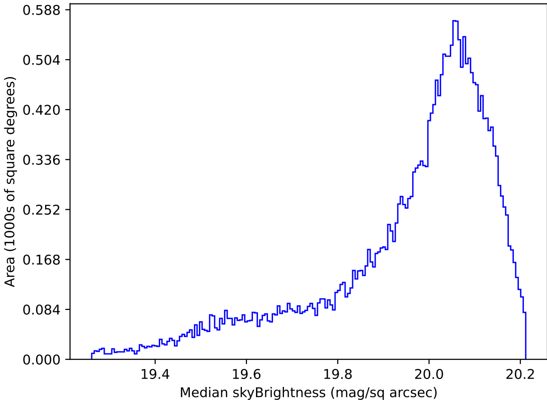
weather_cloudso8v3.4_10yrs All sky i band: Median skyBrightness
