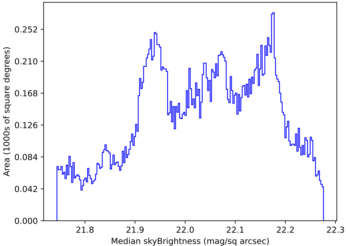
weather_cloudso8v3.4_10yrs All sky g band: Median skyBrightness
