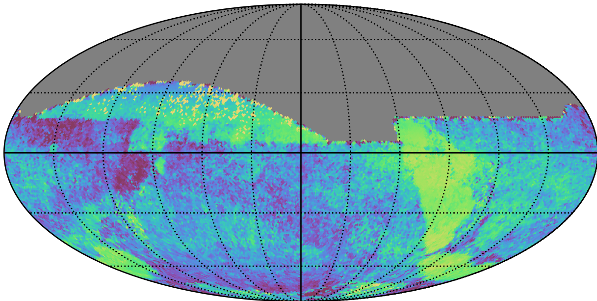
weather_cloudso8v3.4_10yrs All sky all bands: Median skyBrightness
