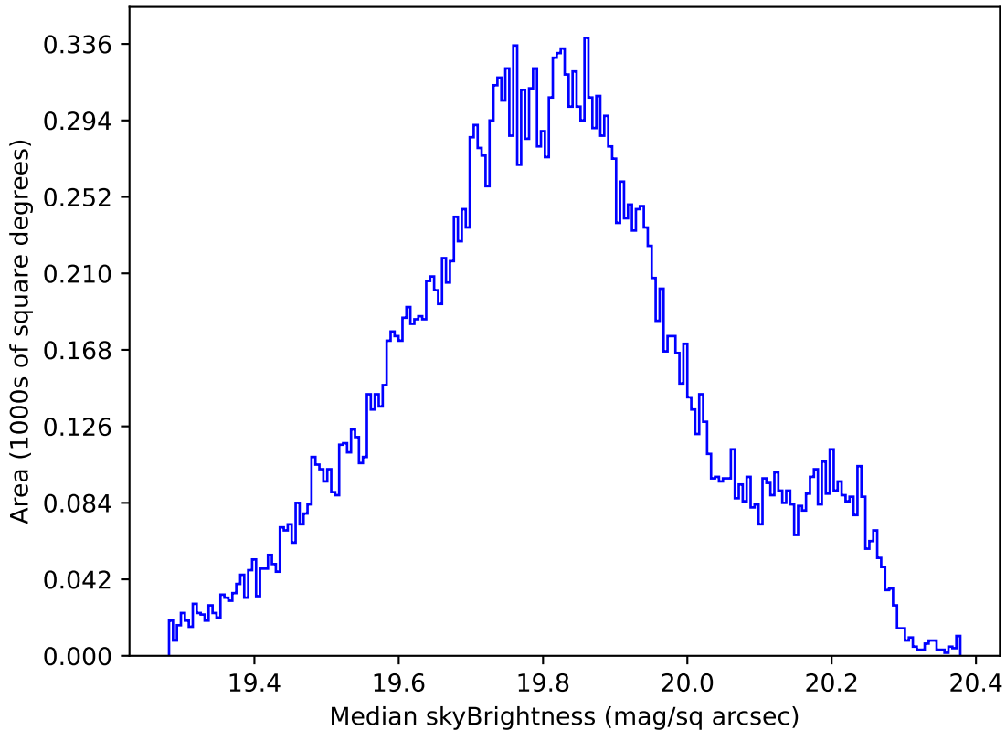
weather_cloudso8v3.4_10yrs All sky all bands: Median skyBrightness
