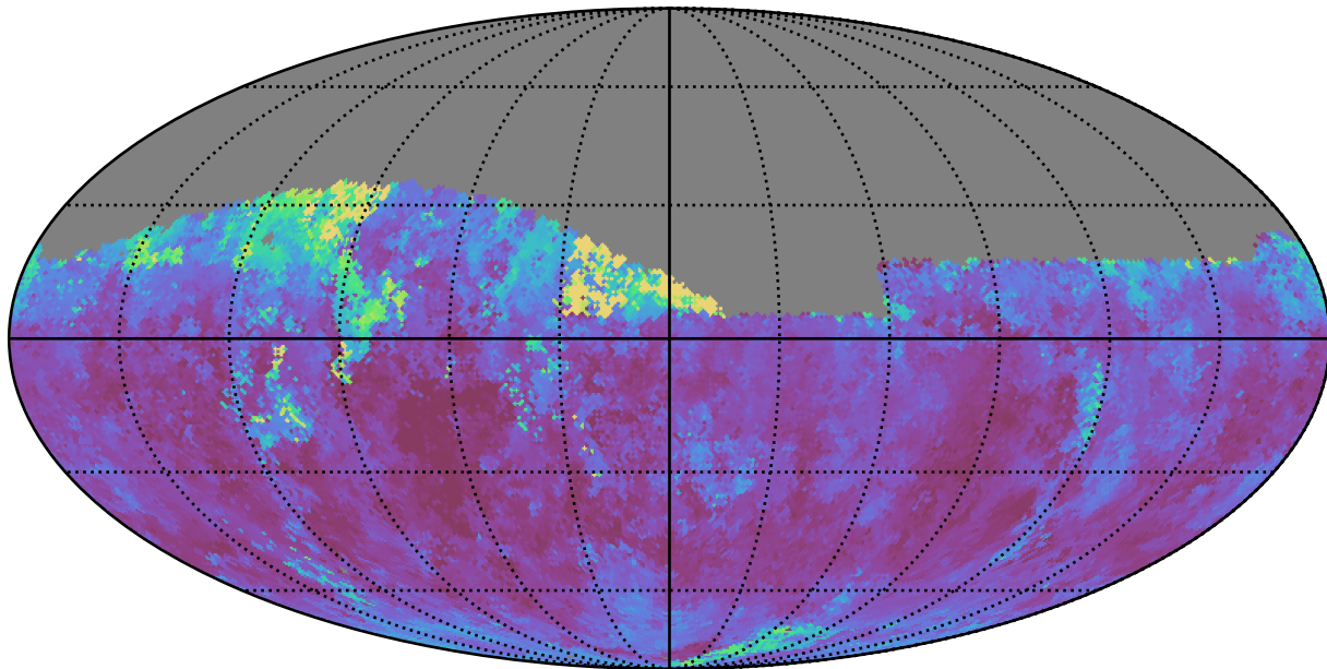
weather_cloudso8v3.4_10yrs Yr 1 z band: Median seeingGeom
