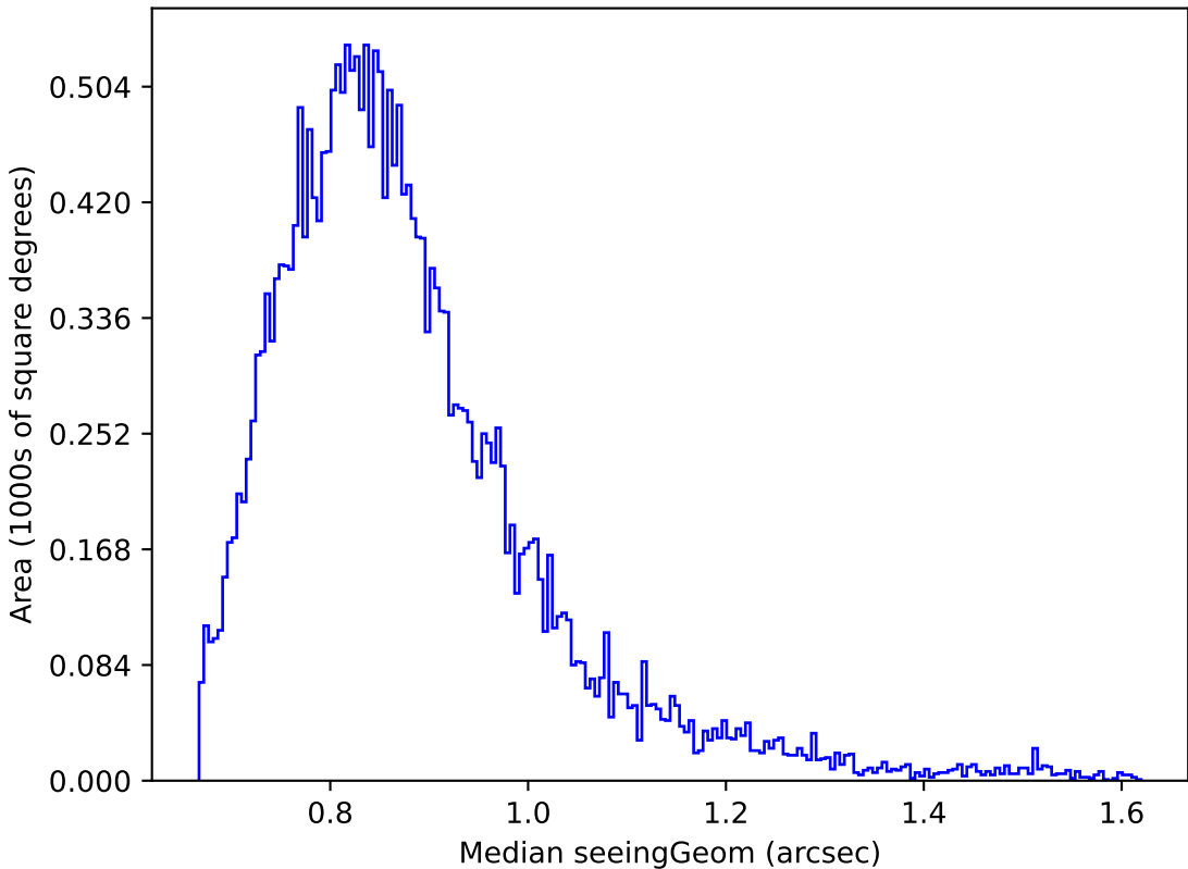
weather_cloudso8v3.4_10yrs Yr 1 z band: Median seeingGeom
