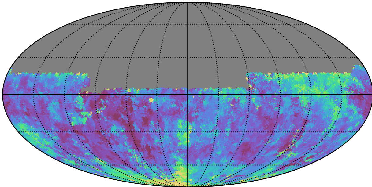
weather_cloudso8v3.4_10yrs Yr 1 y band: Median seeingGeom
