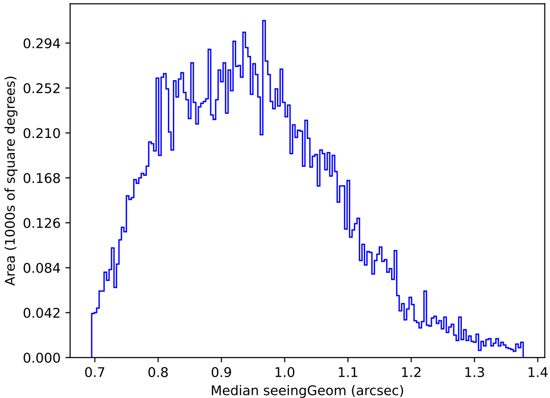
weather_cloudso8v3.4_10yrs Yr 1 u band: Median seeingGeom
