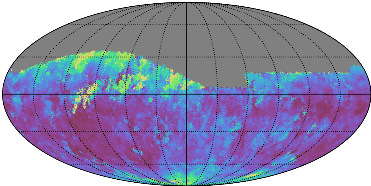
weather_cloudso8v3.4_10yrs Yr 1 r band: Median seeingGeom
