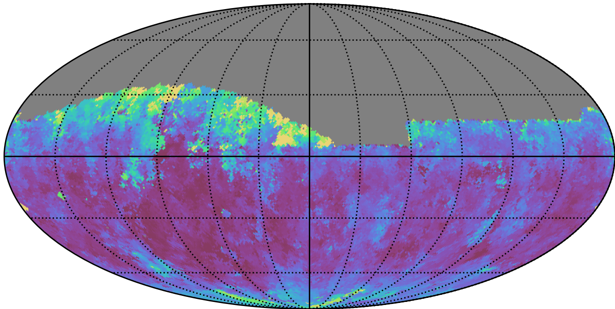
weather_cloudso8v3.4_10yrs Yr 1 i band: Median seeingGeom
