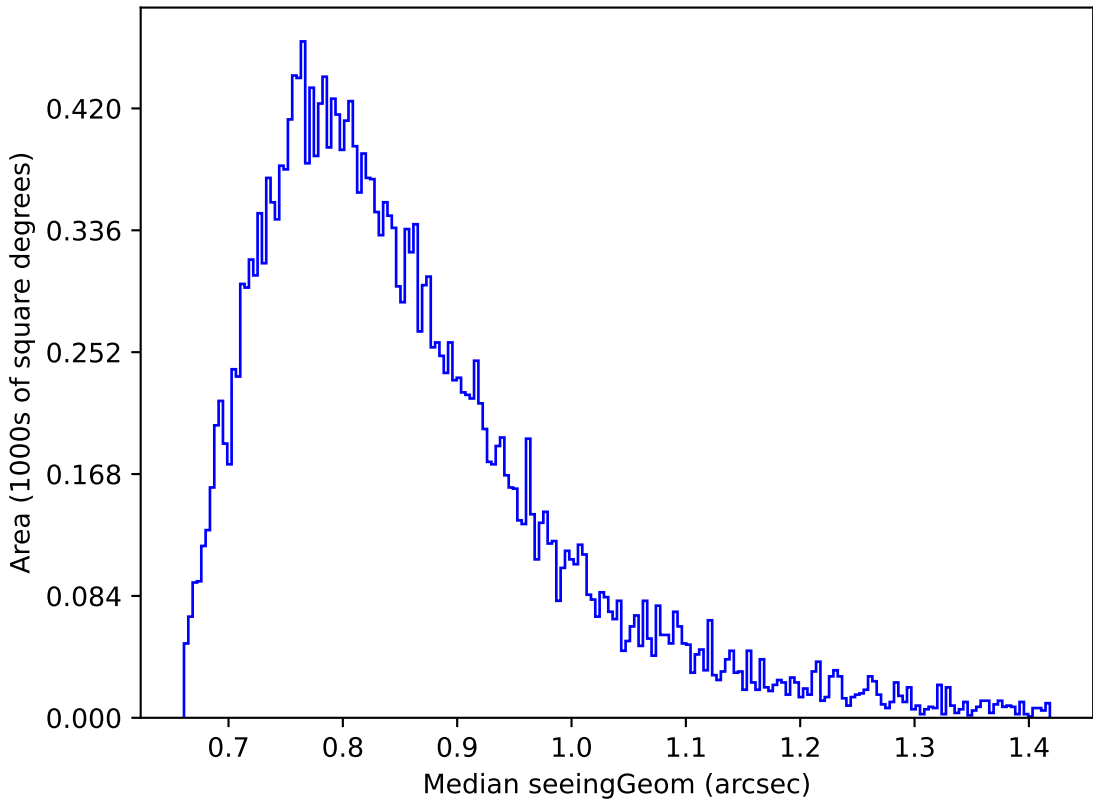
weather_cloudso8v3.4_10yrs Yr 1 i band: Median seeingGeom
