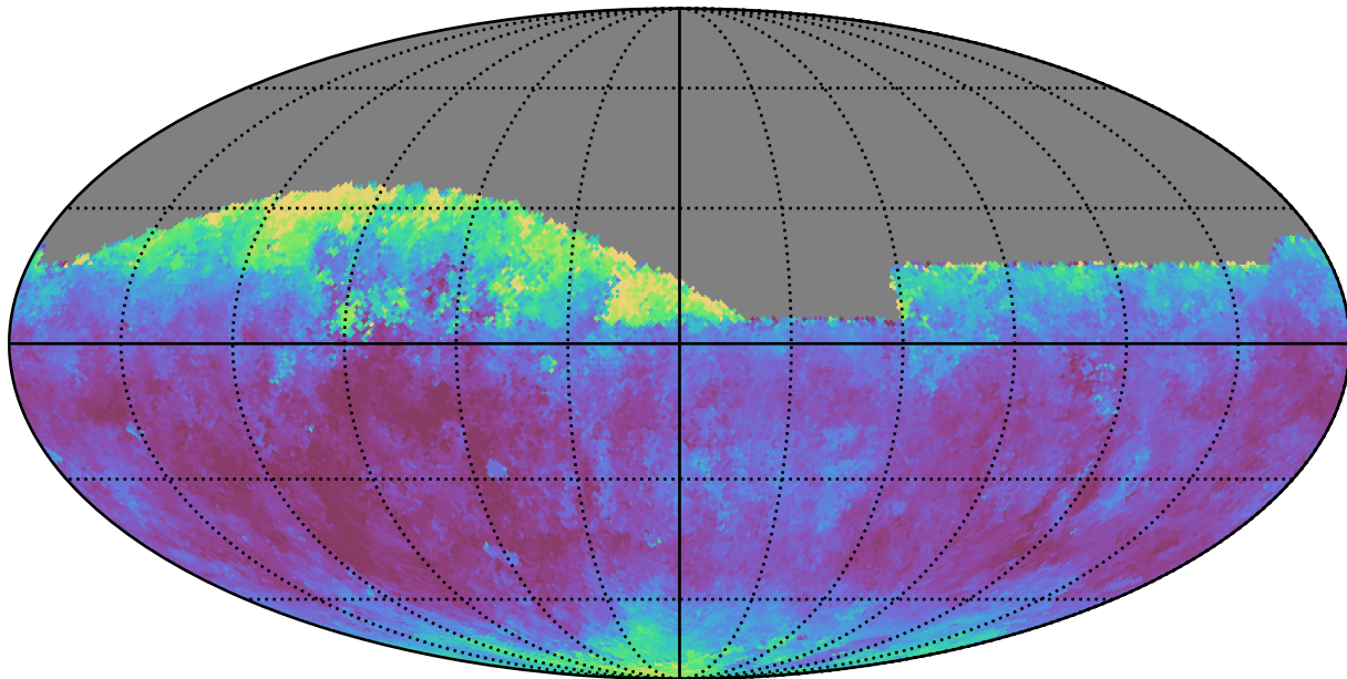
weather_cloudso8v3.4_10yrs Yr 1 all bands: Median seeingGeom
