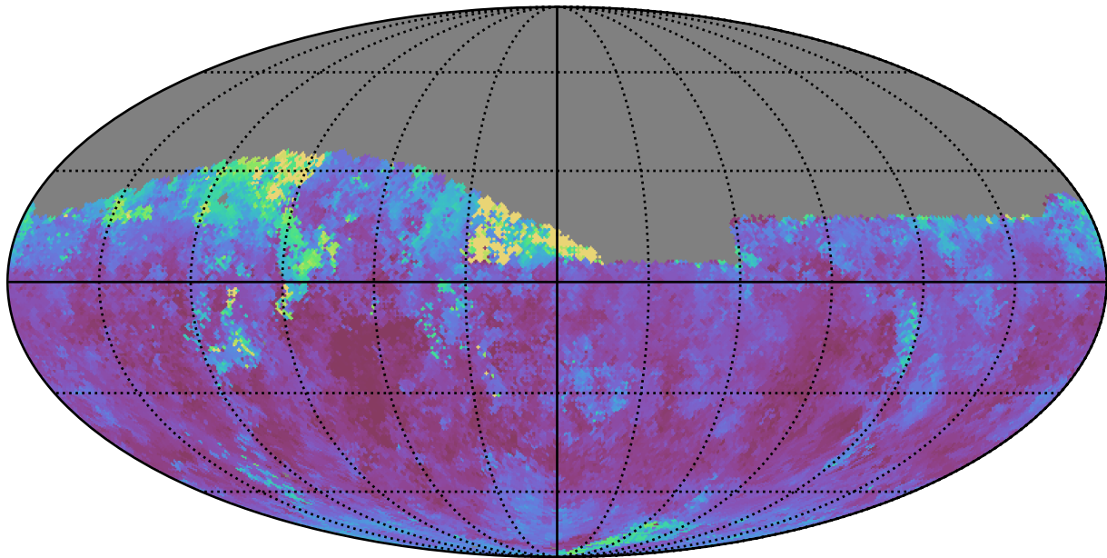
weather_cloudso8v3.4_10yrs Yr 1 z band: Median seeingEff
