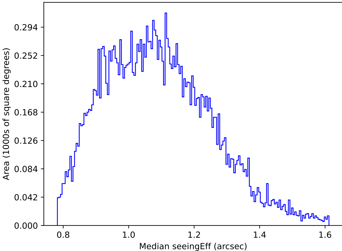
weather_cloudso8v3.4_10yrs Yr 1 u band: Median seeingEff
