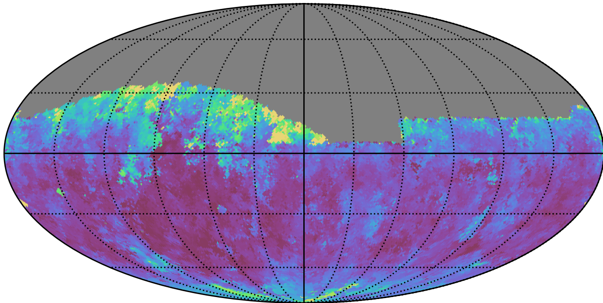
weather_cloudso8v3.4_10yrs Yr 1 i band: Median seeingEff
