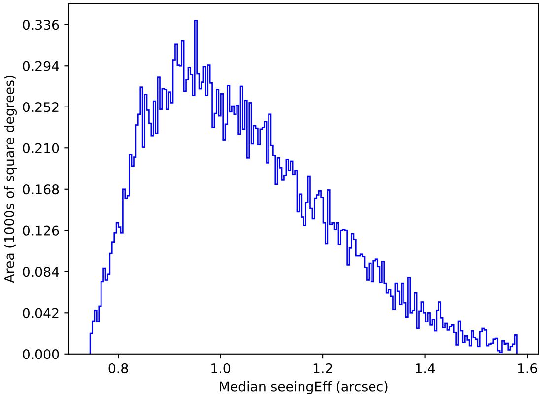
weather_cloudso8v3.4_10yrs Yr 1 g band: Median seeingEff
