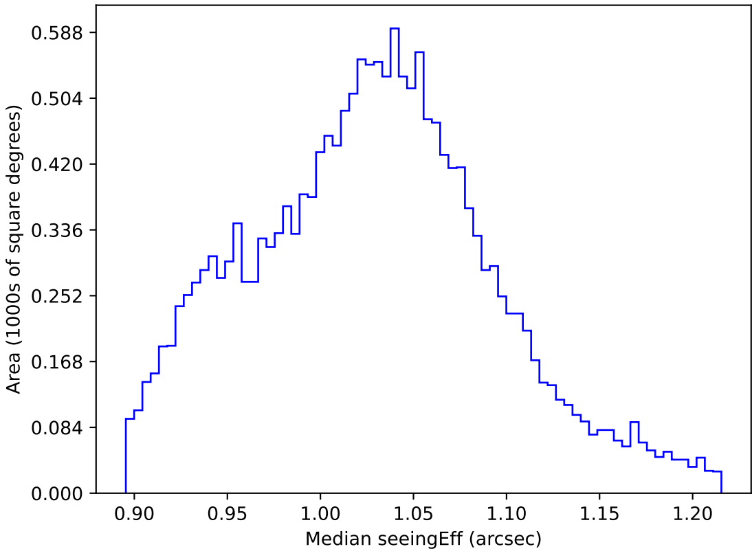
weather_cloudso8v3.4_10yrs WFD z band: Median seeingEff
