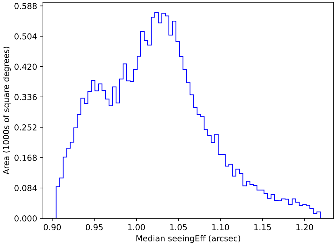
weather_cloudso8v3.4_10yrs WFD y band: Median seeingEff
