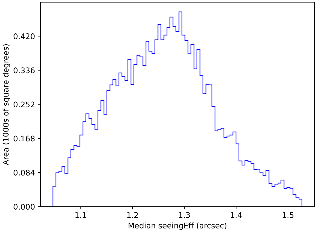
weather_cloudso8v3.4_10yrs WFD u band: Median seeingEff
