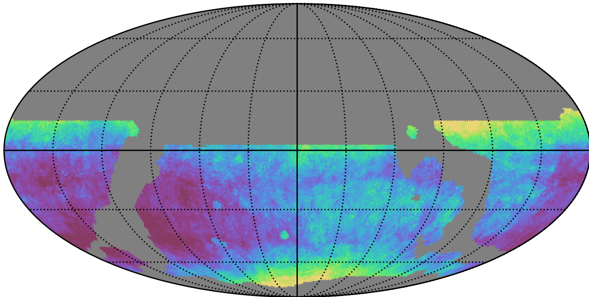
weather_cloudso8v3.4_10yrs WFD i band: Median seeingEff
