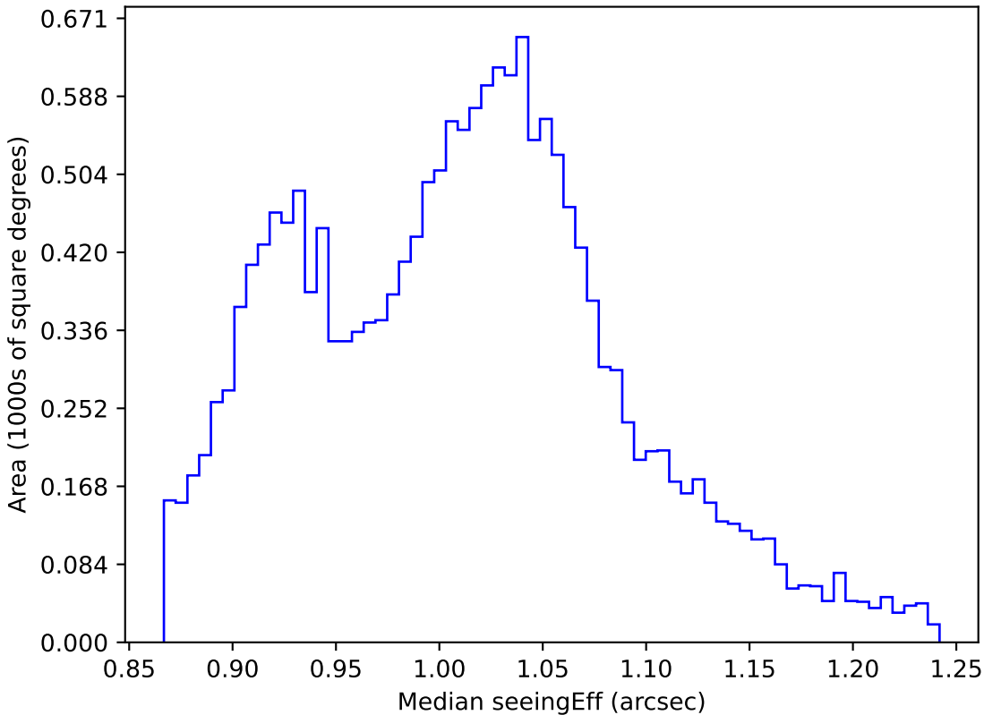
weather_cloudso8v3.4_10yrs WFD i band: Median seeingEff
